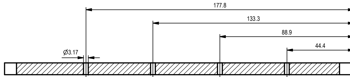
SECTION B-B SCALE 1 / 1.5
