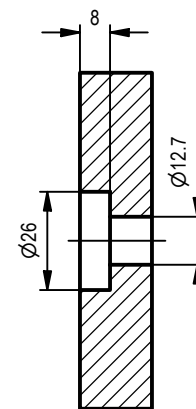
SECTION B-B SCALE 1/2
