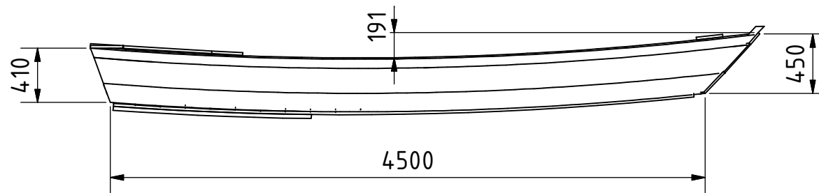
ELEVATION ( 1 : 40 )
