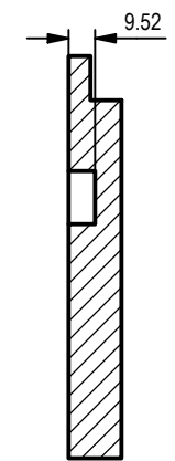
SECTION MD-MD SCALE 1 / 3
