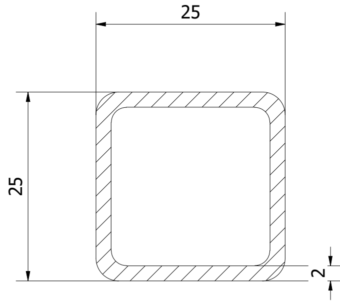
F-F ( 2/1 )
