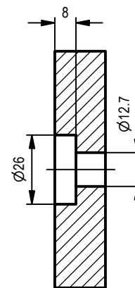
SECTION B-B SCALE 1/2
