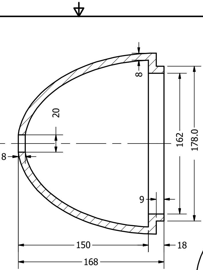
SECTION B-B
